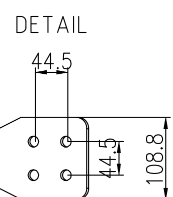
LV BUSHING TERMINAL
